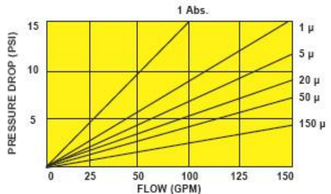
Filter Pressure Drop by Filter Size
